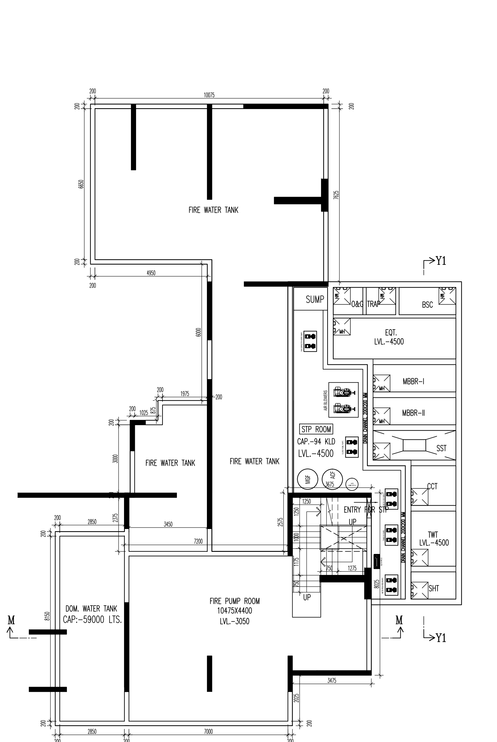
DETAIL OF FIRE PUMP ROOM & STP (94 KLD) BLOCK - A FIRE WATER TANK CAPACITY - 3,50,000 LIT
