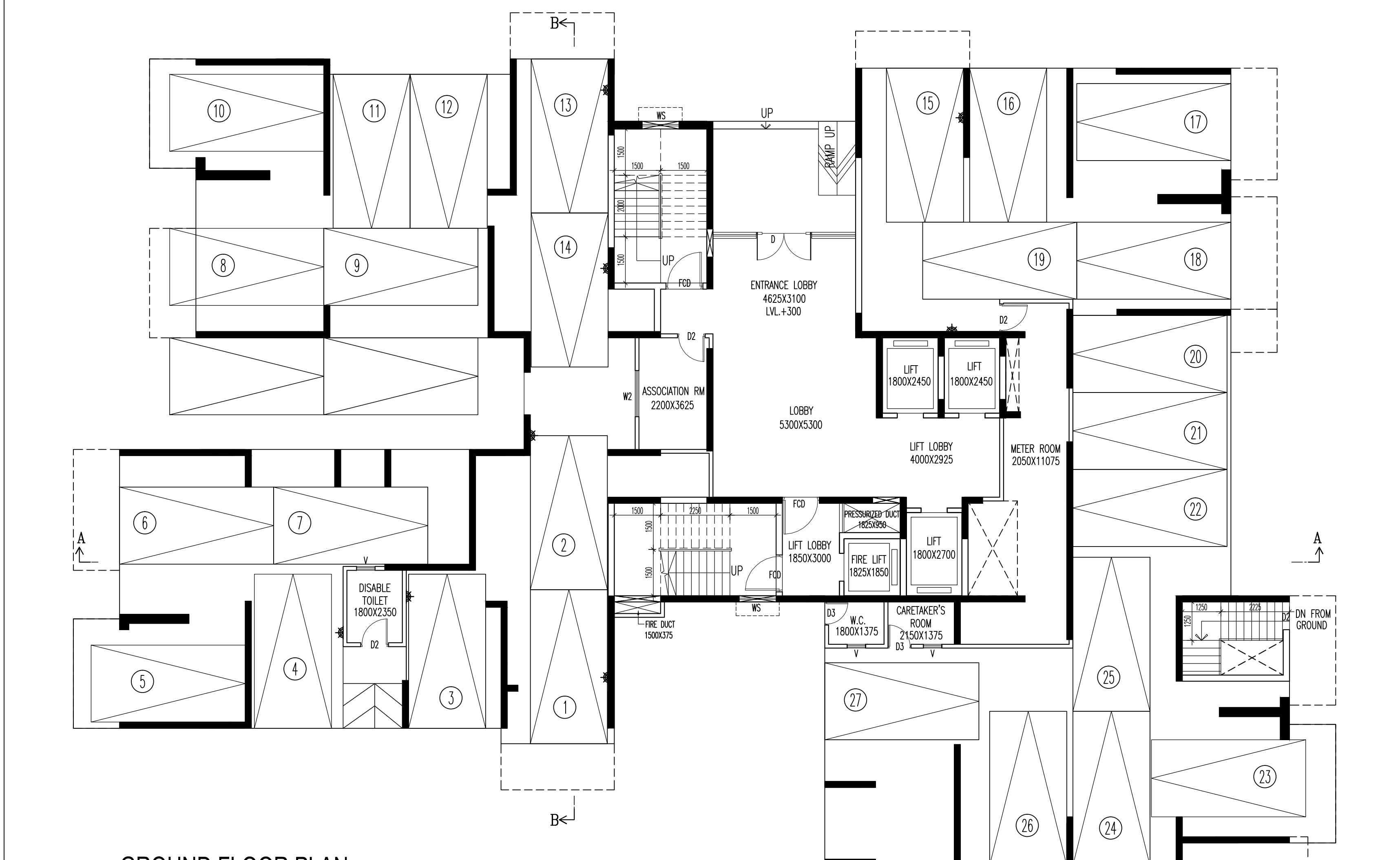
GROUND FLOOR PLAN BLOCK - A
